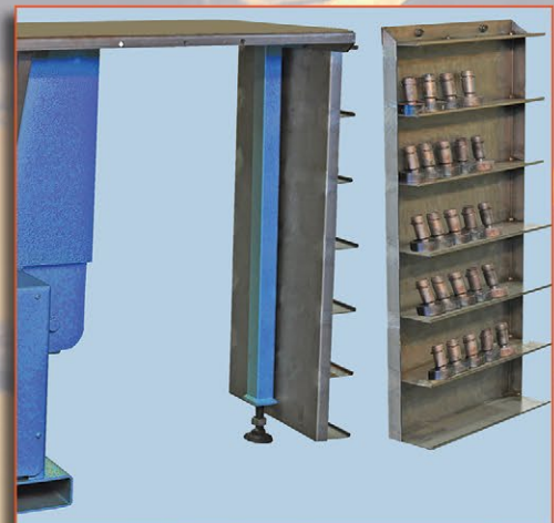
Tool table extension with punch and die storage rack
