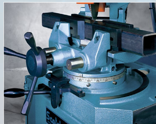
Miter Locking Device
