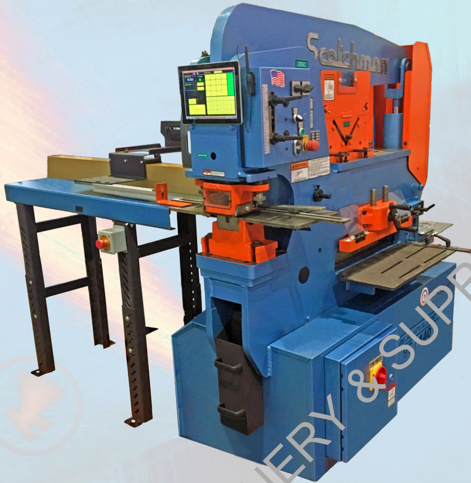
The RG Stop System connected to the punch station of the Scotchman DO 95/140-24M Ironworker
